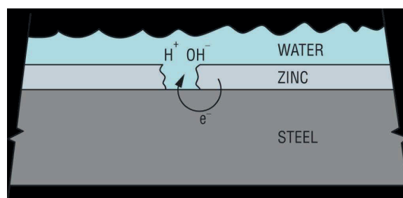
Figure 2 – Production of hydrogen ( H^+ ) from the galvanic protection of steel by a zinc coating
