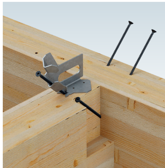
Example of inclined installation - GSCREW4560-R
