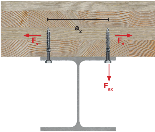
CLT Floor supported above Steel I-Beam
