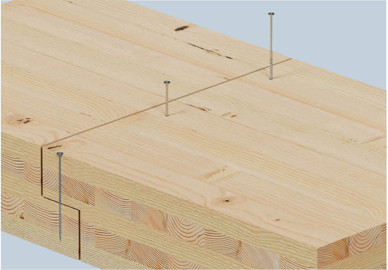
CLT Floor to CLT Floor (in plane connection)
