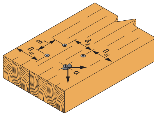
Illustration above shows angle between load direction and grain = 90^\circ
