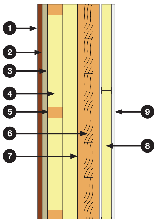
Horizontal cladding and internal lining isolated from the wall
