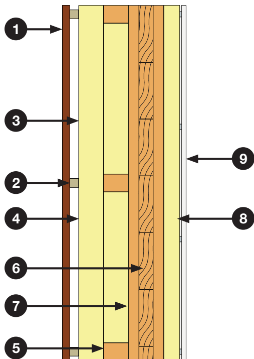
Vertical cladding and internal structure fixed to the wall
